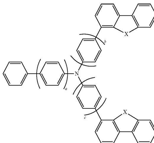
Chemical Formula 2
