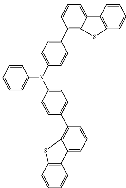
Chemical Formula 1-6
