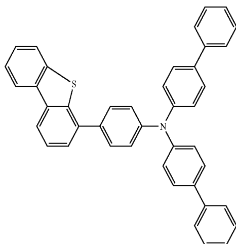
Chemical Formula 1-6
