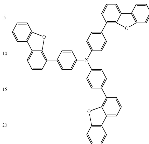
Chemical Formula 1-1
