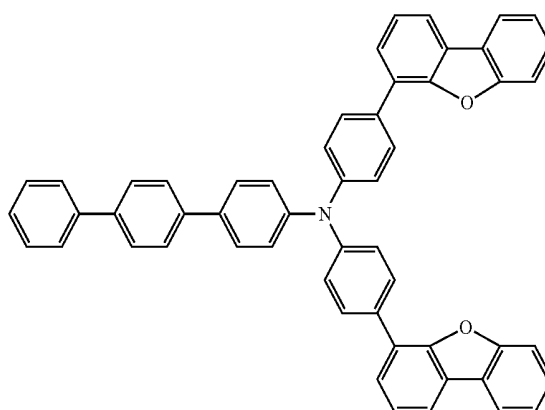
Chemical Formula 2-1
