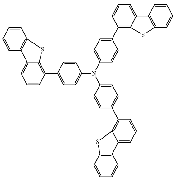
Chemical Formula 1-5
