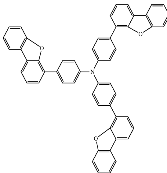
Chemical Formula 1-2
